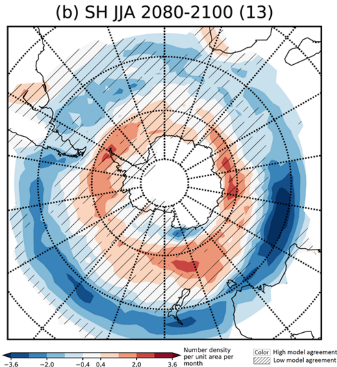
Figure 4: Changes in extratropical storm track density over the Southern Hemisphere. Displayed is the projected spatial pattern of multi-model mean change of extratropical storm track density in winter (SH JJA) in 2080–2100 for SSP5-8.5 relative to 1979–2014 based on 13 CMIP6 models. Hatching indicates regions where fewer than 80% of the models agree on the sign of the change and no overlay where at least 80% of the models agree on the sign of change. Units are number density per 5-degree spherical cap per month. From IPCC AR6 WG1 Report, Figure 4.27.
