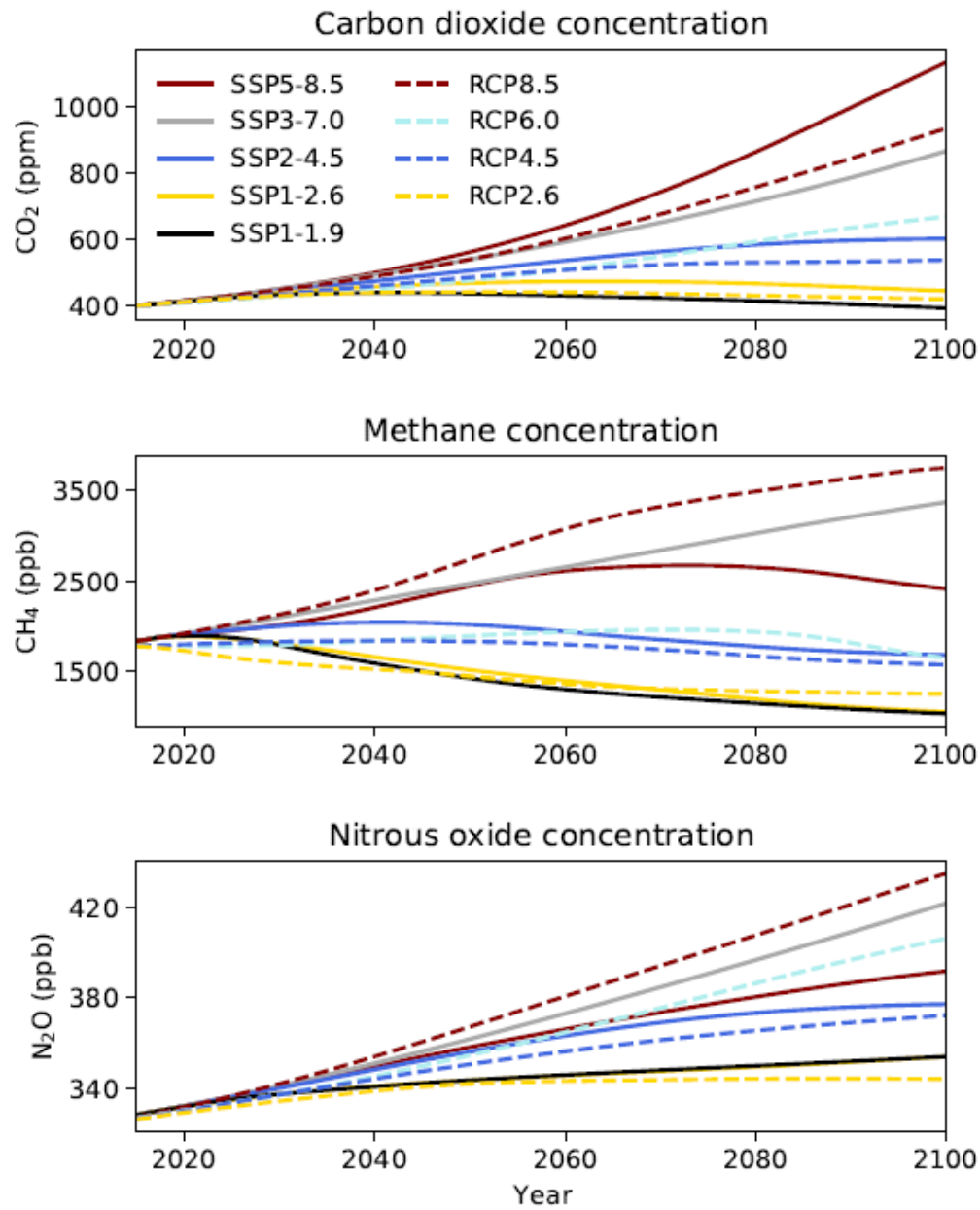
Figure 1: Global, annual-mean greenhouse gas concentrations in the Shared Socioeconomic Pathways (SSPs, solid lines) and Representative Concentration Pathways (RCPs, dashed lines). Data sourced from Meinshausen et al. (2011) and Meinshausen et al. (2020).
