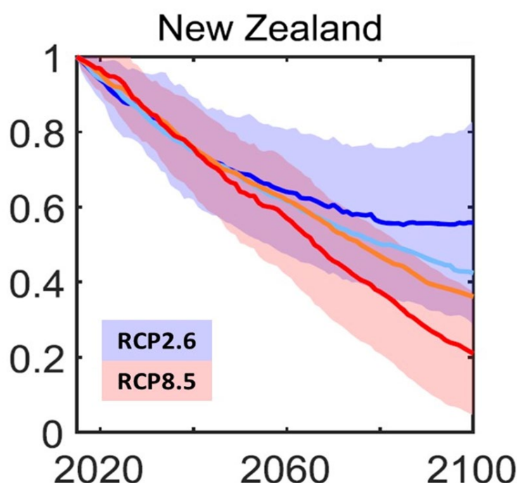
Figure 7. Glacier mass relative to 2015 as a function of time and RCP scenario. Solid lines indicate ensemble median and shading indicates ±1 standard deviation (shown only for RCP2.6 and RCP8.5 for clarity). (Source: Modified Figure 6 from Marzeion et al. , 2020).
