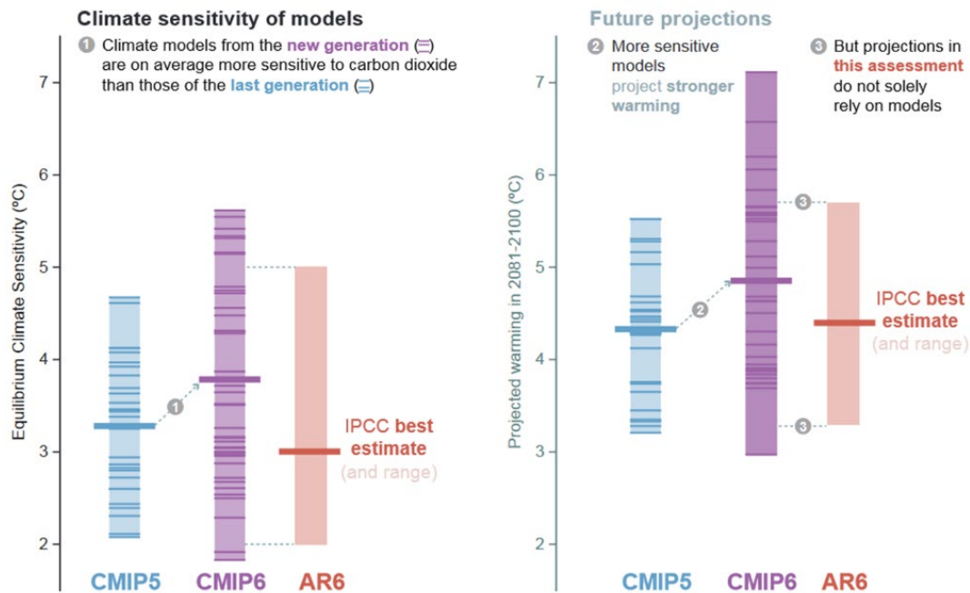
Figure 2: Climate sensitivity and future warming. Left: Equilibrium climate sensitivities for the current CMIP6 and the previous CMIP5 generations of climate models, and the best estimate and very likely range as assessed in IPCC AR6. Right: Same, but for the end-of-century (2081-2100) warming under the RCP8.5 and SSP5-8.5 scenarios, respectively. (reproduced from IPCC AR6, FAQ 7.3, figure 1).
