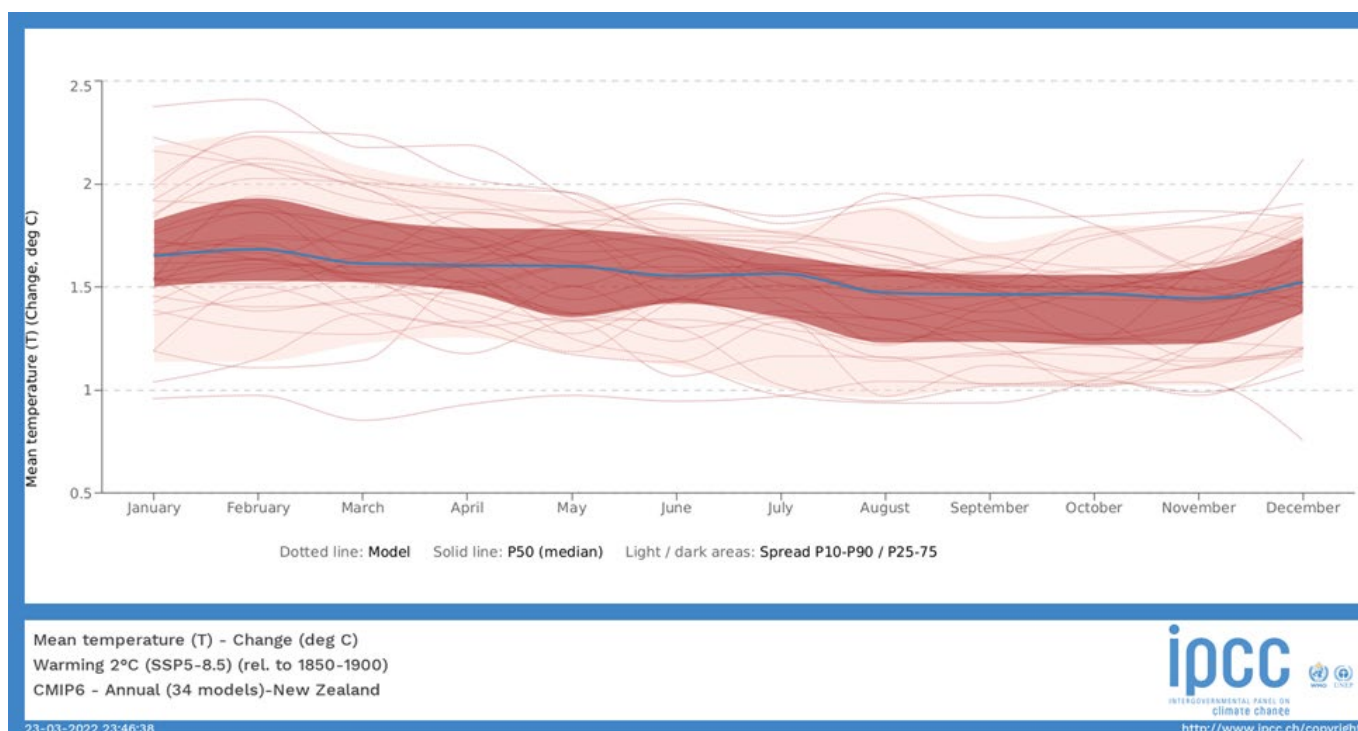
Figure 5: Seasonal temperature projection for the New Zealand region (derived from the IPCC WG1 Atlas).
